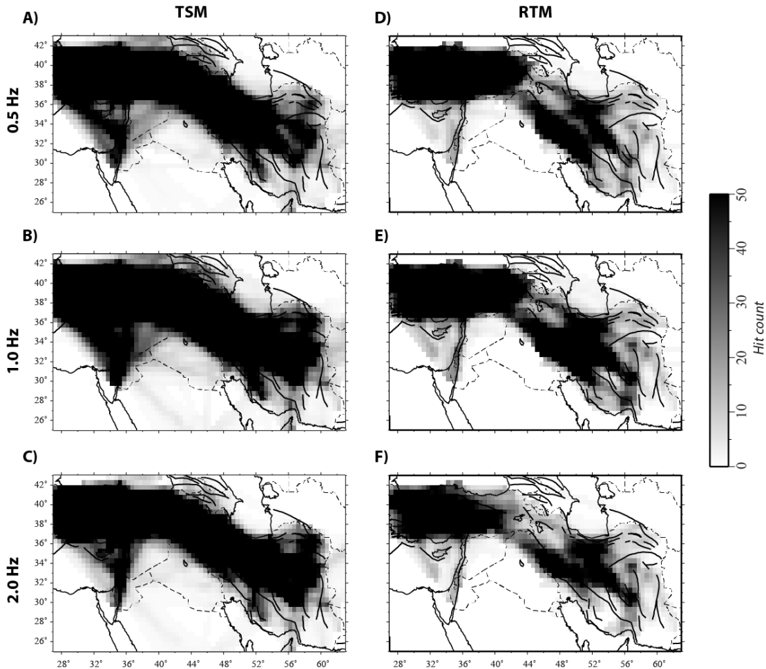
Figure S1. Maps showing ray coverage per model block. The darker the region, the higher is the hit count.
