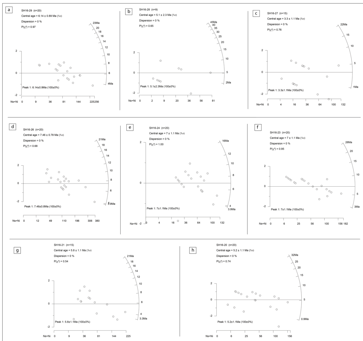
Figure S2. Radial plots for AFT samples from the Tilcara Range, Cianza area and east side of the Eastern Cordillera.
