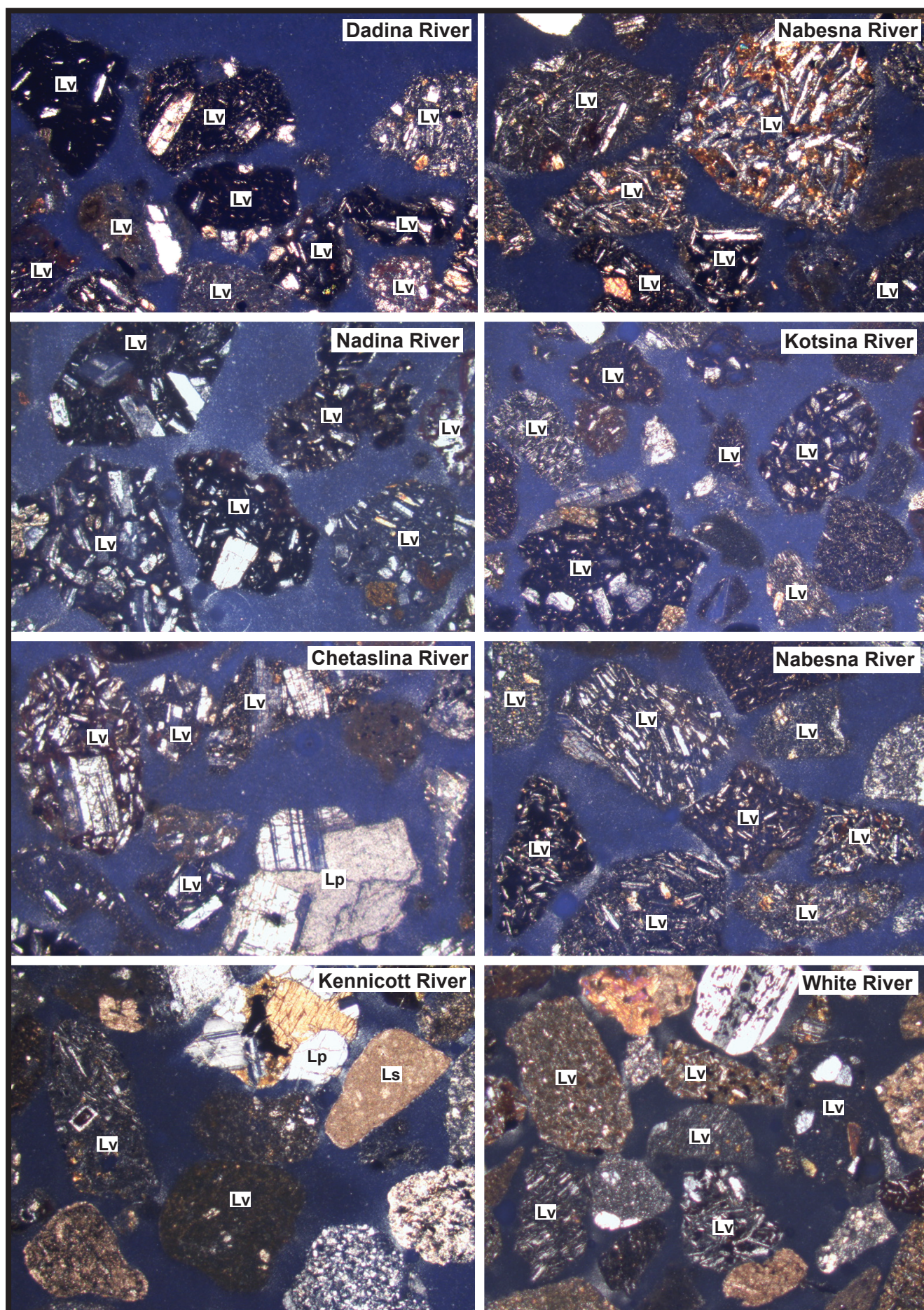
Supplemental Item S2 - Photomicrographs of representative modern river sand samples showing abundant volcanic lithic grains (Lv), especially lathwork varieties, and subordinate plutonic (Lp) and sedimentary (Ls) lithic grains. All images in cross-polarized light. Refer to Table 1 and Figure 3 for sample locations.
