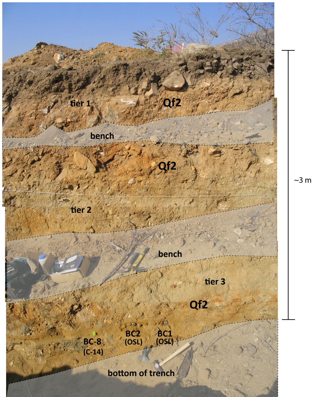
Figure S3: Photomosaic of the northern end of trench WT-3C, showing the locations of dated luminescence sample BC2 and dated radiocarbon sample BC-8 from a ~10-cm-thick sand layer within Qf2. Luminescence sample BC1 could not be dated. View to west. See Figure 3 for locations of these samples in map-view.
