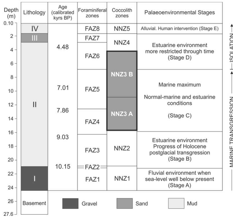
Figure S1: Summary of lithostratigraphic units, micropalaeontological zones and palaeoenvironmental stages throughout the MIRA-CP1 core (modified from Alday et al., 2006)
