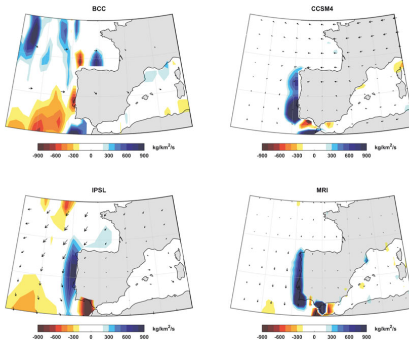
Figure S6: Anomalies in the summer Upward Mass Transport of water in the 0-150 m layer (shaded) and in surface wind (vectors) over the INAM during the mid-Holocene (when compared to the pre-industrial control period) from four atmosphere-ocean coupled general circulation models (CGCMs) that contributed to the third phase of the Paleoclimate Modelling Intercomparison Project (PMIP3; Braconnot et al. 2012 ) within the scope of CMIP5. These models are: (i) BCC-CSM1.1 ( Xin et al. 2013 ), (ii) CCSM4 ( Gent et al. 2011 ), (iii) IPSL-CM5A-LR ( Dufresne et al. 2013 ) and (iv) MRI-CGCM3 ( Yukimoto et al. 2012 ).
