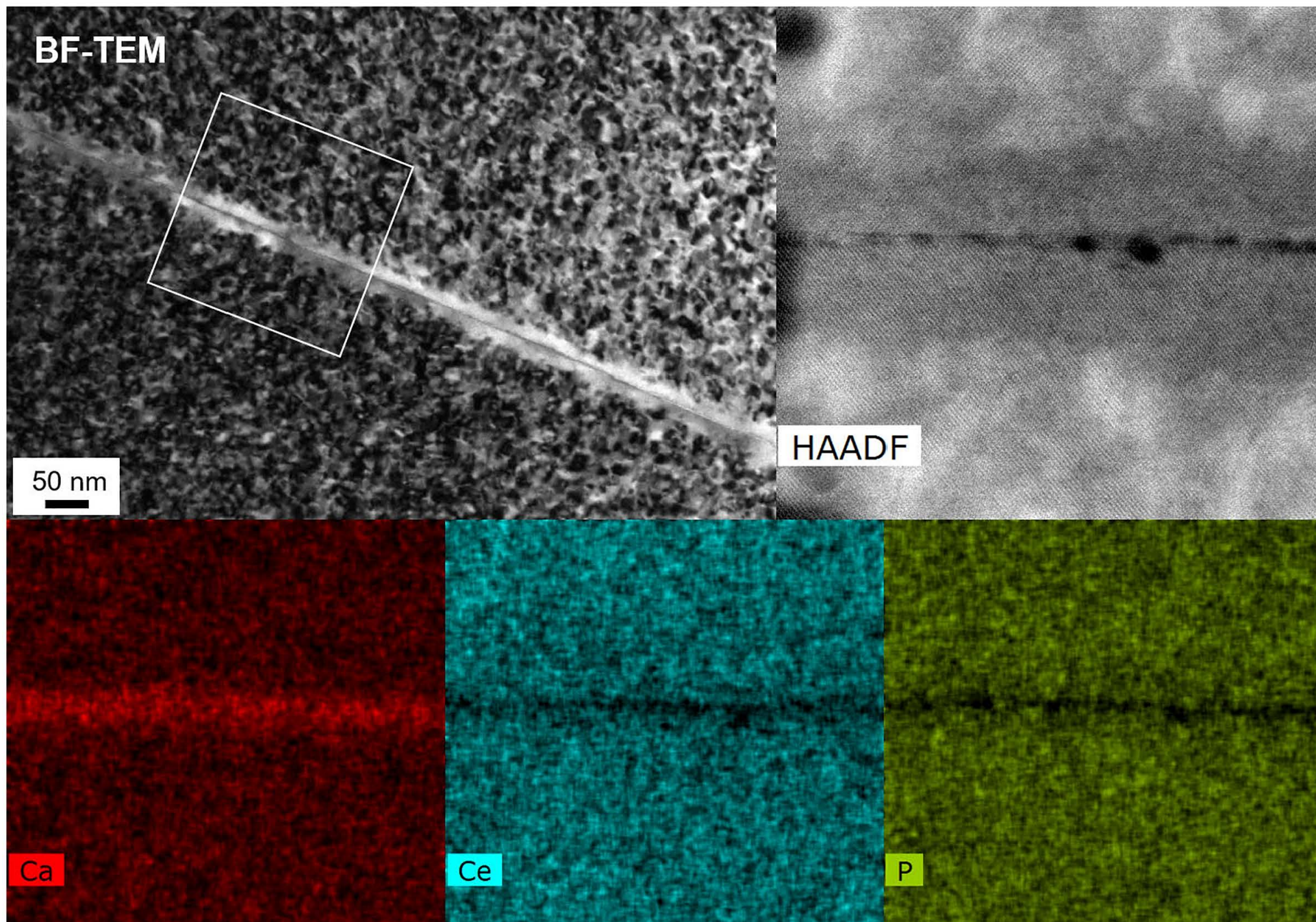
Figure S2. Bright field TEM image and EDS data
