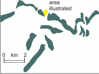
PLATE DR2: GSA Data Repository Item 2019211 accompanies Keighley, D., Spinnangr, Ø., Howell, J., and Flint, S., 2019, Interpretation of mouth-bar and related lacustrine and fluvial sand bodies from the middle Green River Formation (Eocene), southern Uinta Basin, Utah, in Starratt, S.W., and Rosen, M.R., eds., From Saline to Freshwater: The Diversity of Western Lakes in Space and Time: Geological Society of America Special Paper 536, https://doi.org/10.1130/2019.2536(15) .
