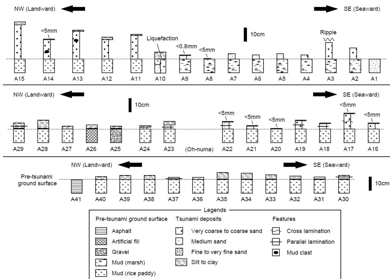
Fig. 10. Columnar sections of the tsunami deposit along survey transect.
