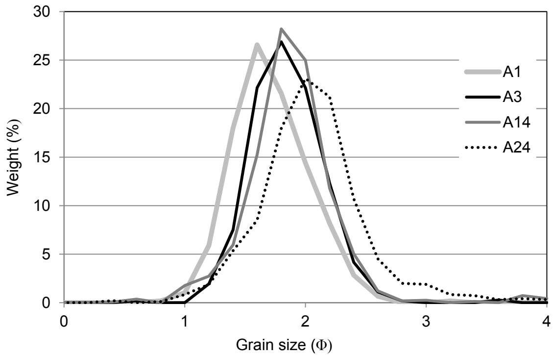
Fig. 7. Grain size distributions of sand deposits at A1 (beach sand, 0.5 km from the shoreline), A3 (2.5 km from the shoreline), A14 (1.35 km from the shoreline), and A24 (2.35 km from the shoreline) along the transect.
