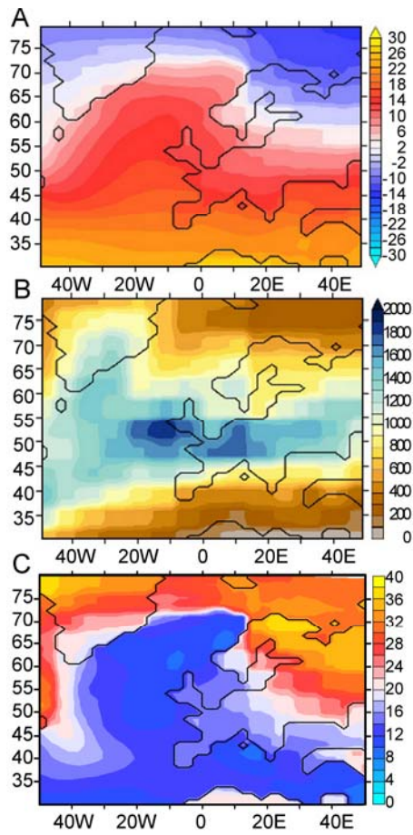
Figure DR2. A. Mean annual surface air temperature (°C), B. Mean annual precipitation (mm), C. Annual temperature range (°C) in Europe for experiment 15Ma560.
