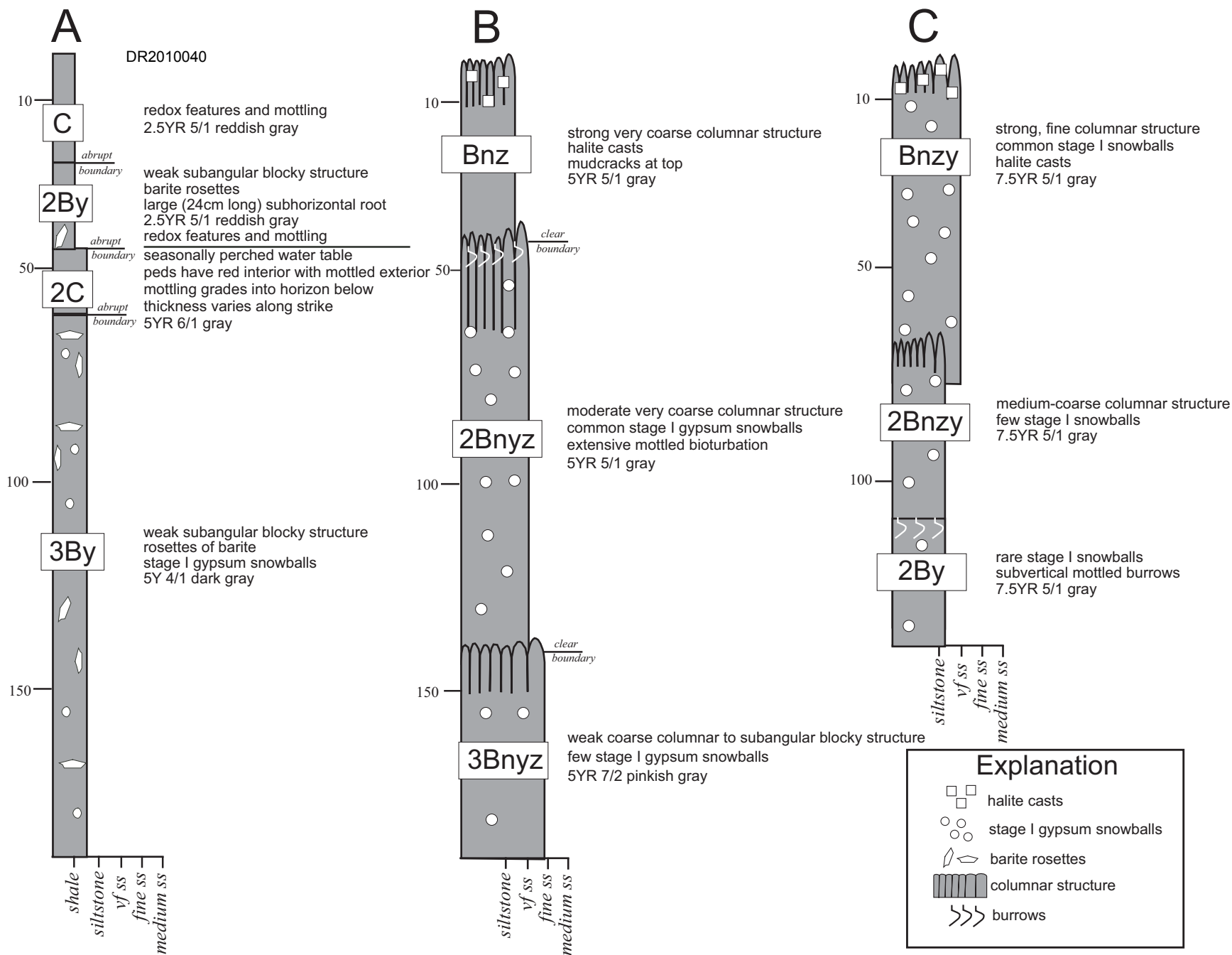
Data Repository Figure 1. Examples of some typical soil horizons present in Carroza Formation. Soil descriptions from: A) soil profile ~420 meters from base of Carroza in Arroyo Las Cabras section, B) soil profile ~220 meters from base of Carroza in Diablo Canyon section, and C) soil profile ~130m from base of Carroza in Diablo Canyon section.
