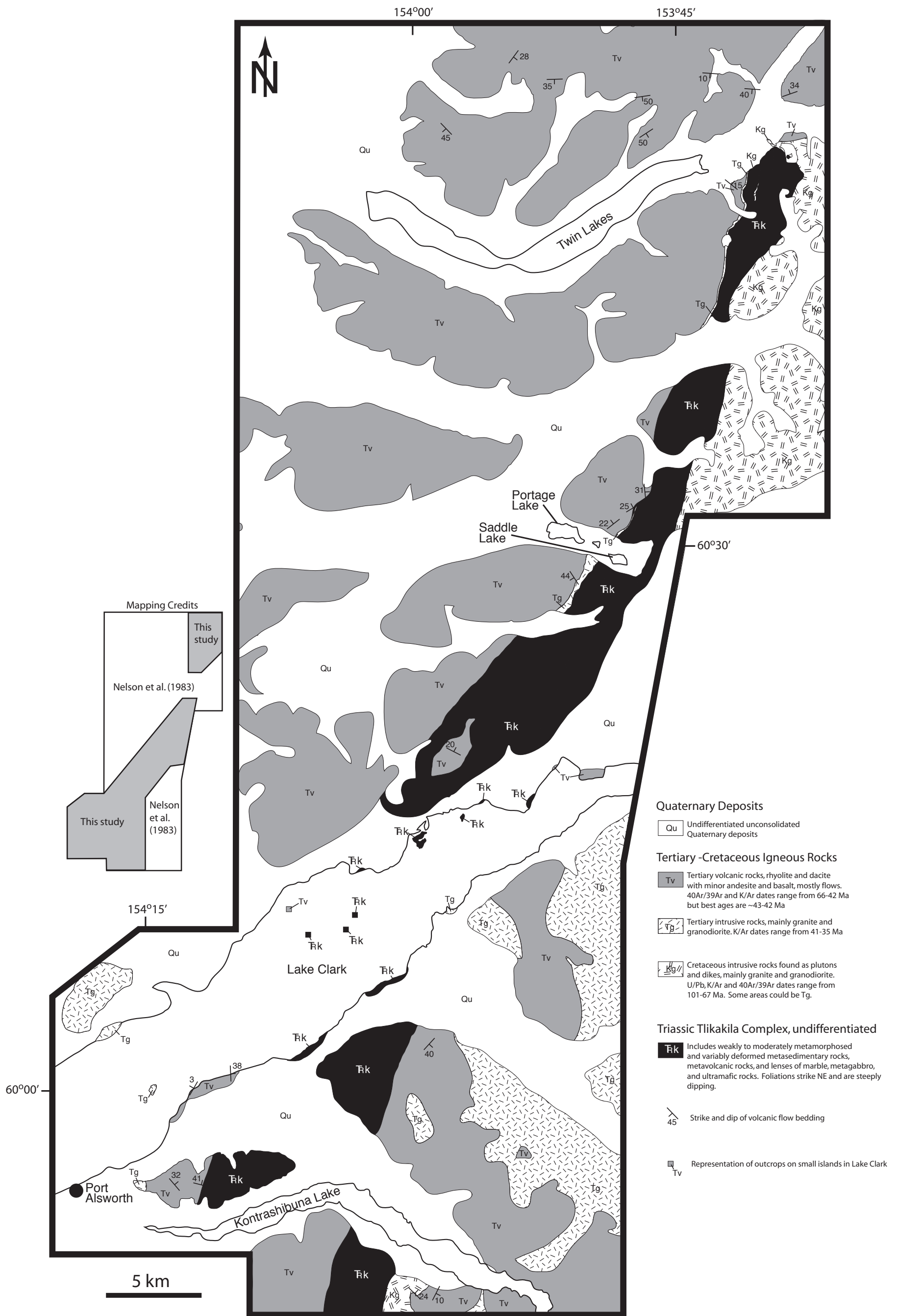
Bedrock Geologic Map of the Tlikakila Complex and Adjacent Rocks of the Lake Clark Region
