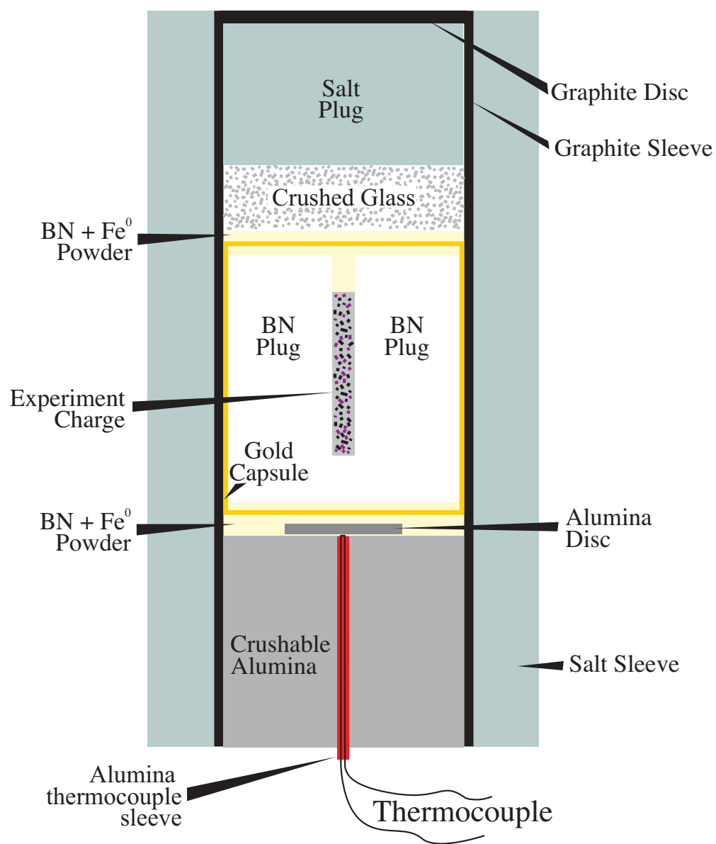
Figure DR2. Design of the experiment assembly used in this study.
