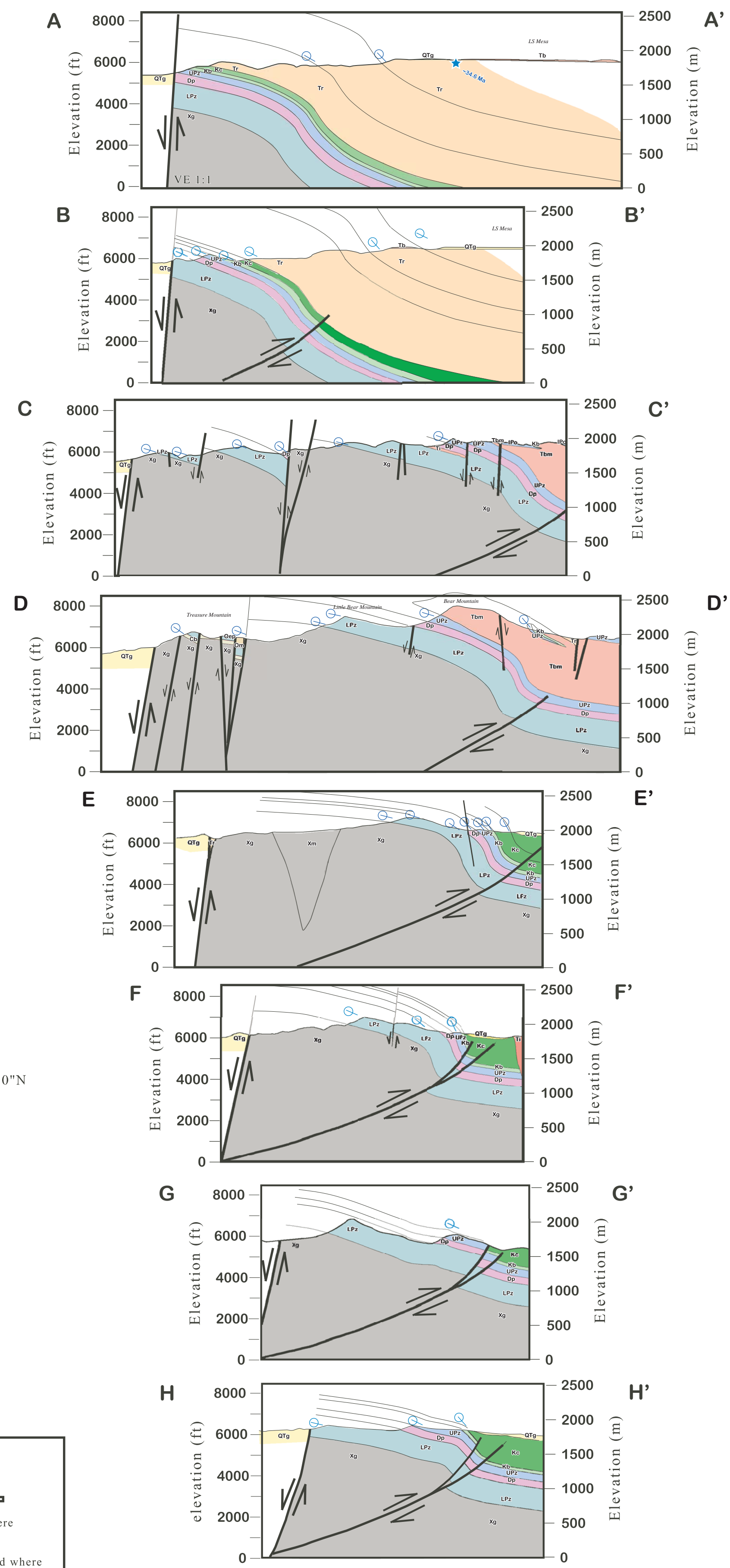
Plate 1. Geologic Map and cross sections of the Silver City Range, Grant County, NM (after Copeland et al. , 2010).
